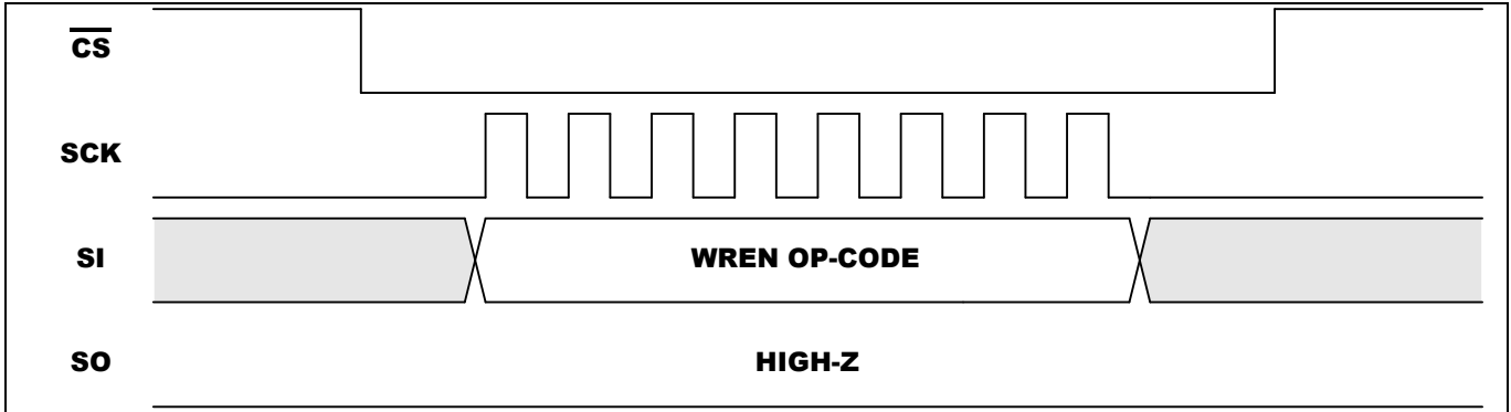
Figure 5-1. WREN Sequence
