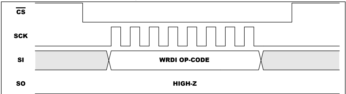
Figure 5-2. WRDI Sequence
