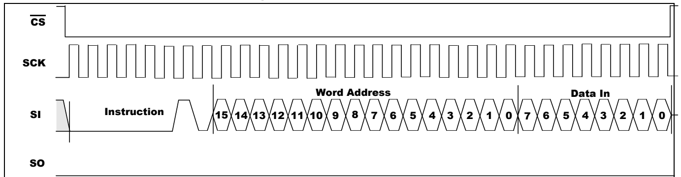
Figure 5-6. WRITE Sequence
